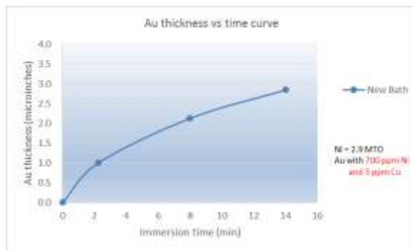
FIGURE 6. PLATING RATE FOR NEW BATH
